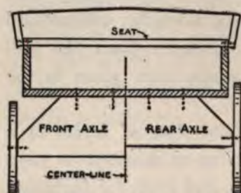
FIG. 286. — Cross-Section of the Express-Wagon.
